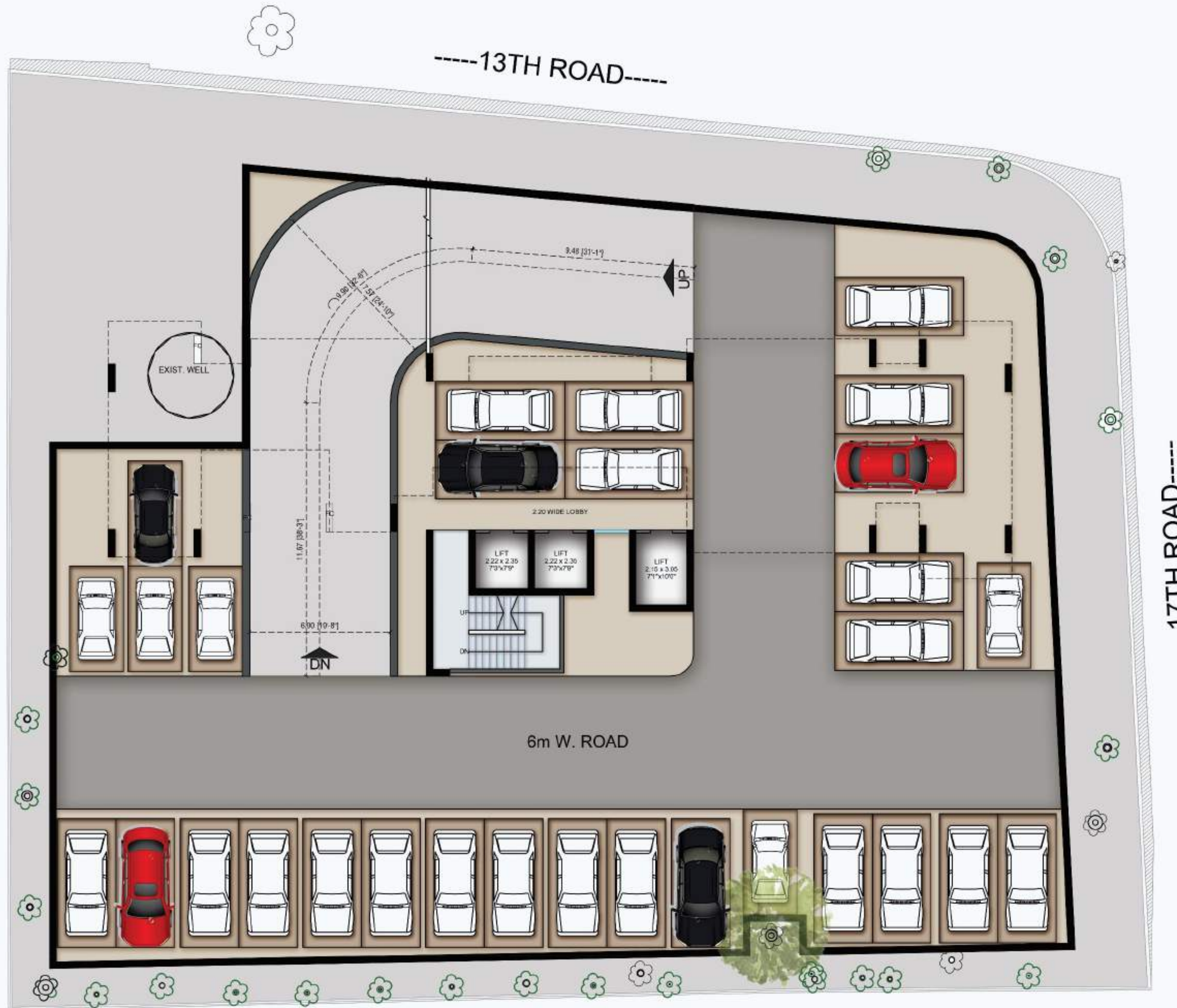
2 ND BASEMENT FLOOR PLAN
