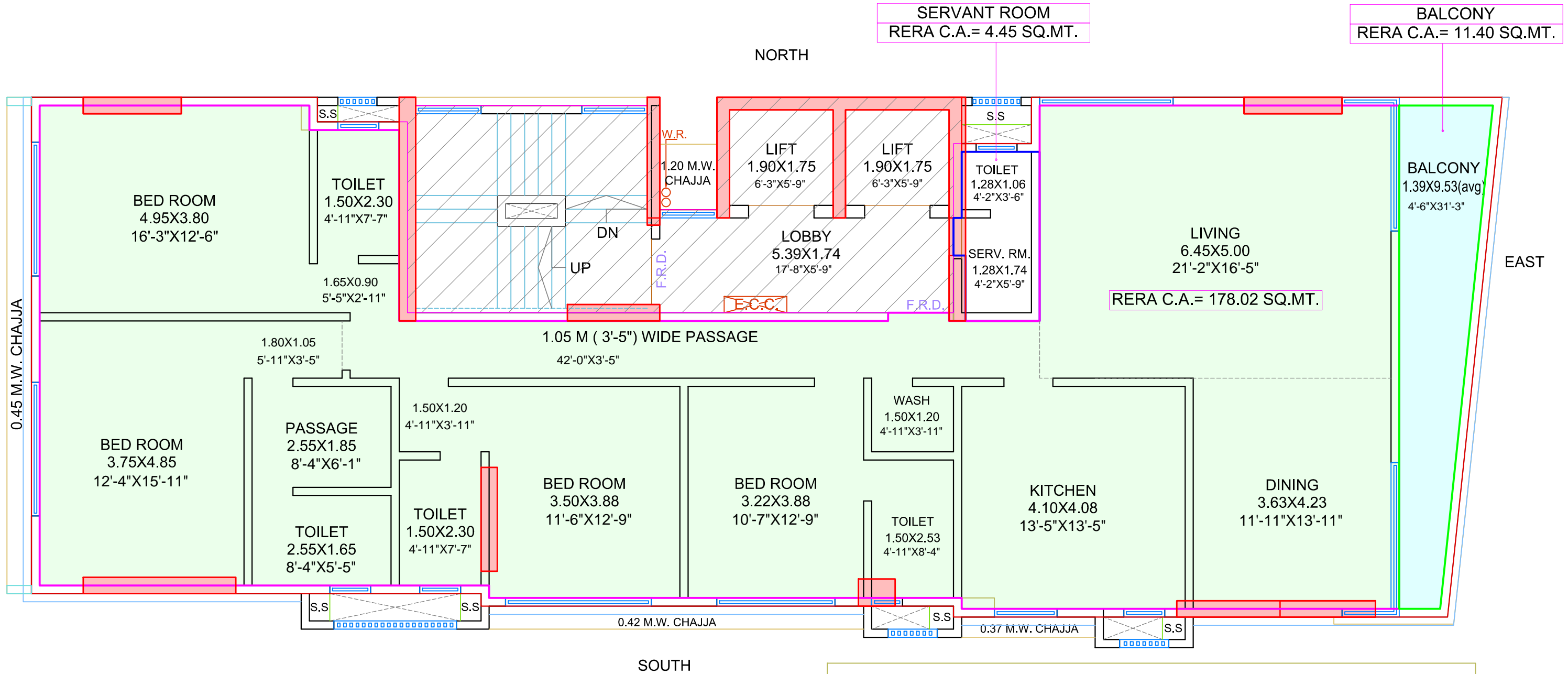
TYPICAL 8TH TO 13TH & 15TH FLOOR PLAN SCALE :- 1:100
